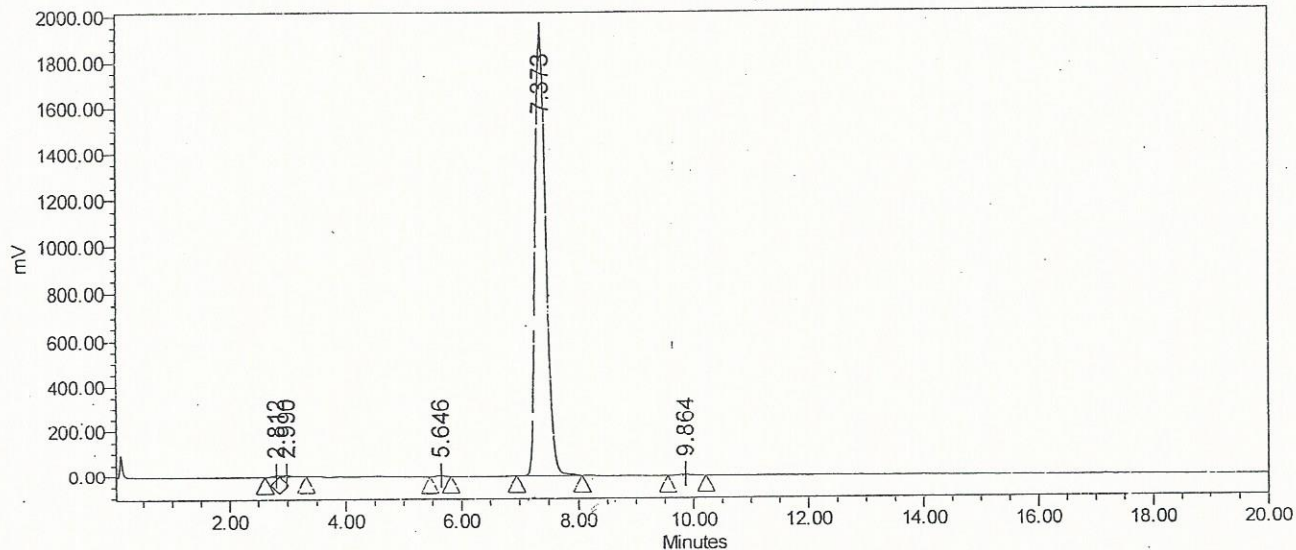
Auto-Scaled Chromatogram
